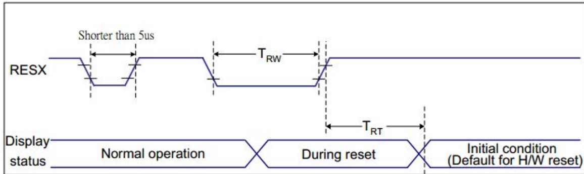
Figure 7 Reset Timing
