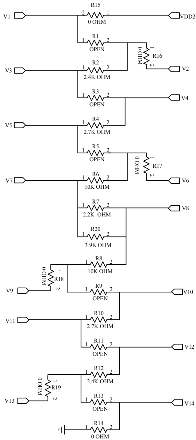
Note 5-10: Typical Application Circuit (When VDD2 = +9.5V)
