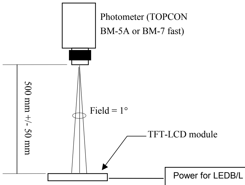
Optical characteristics measuring configuration
