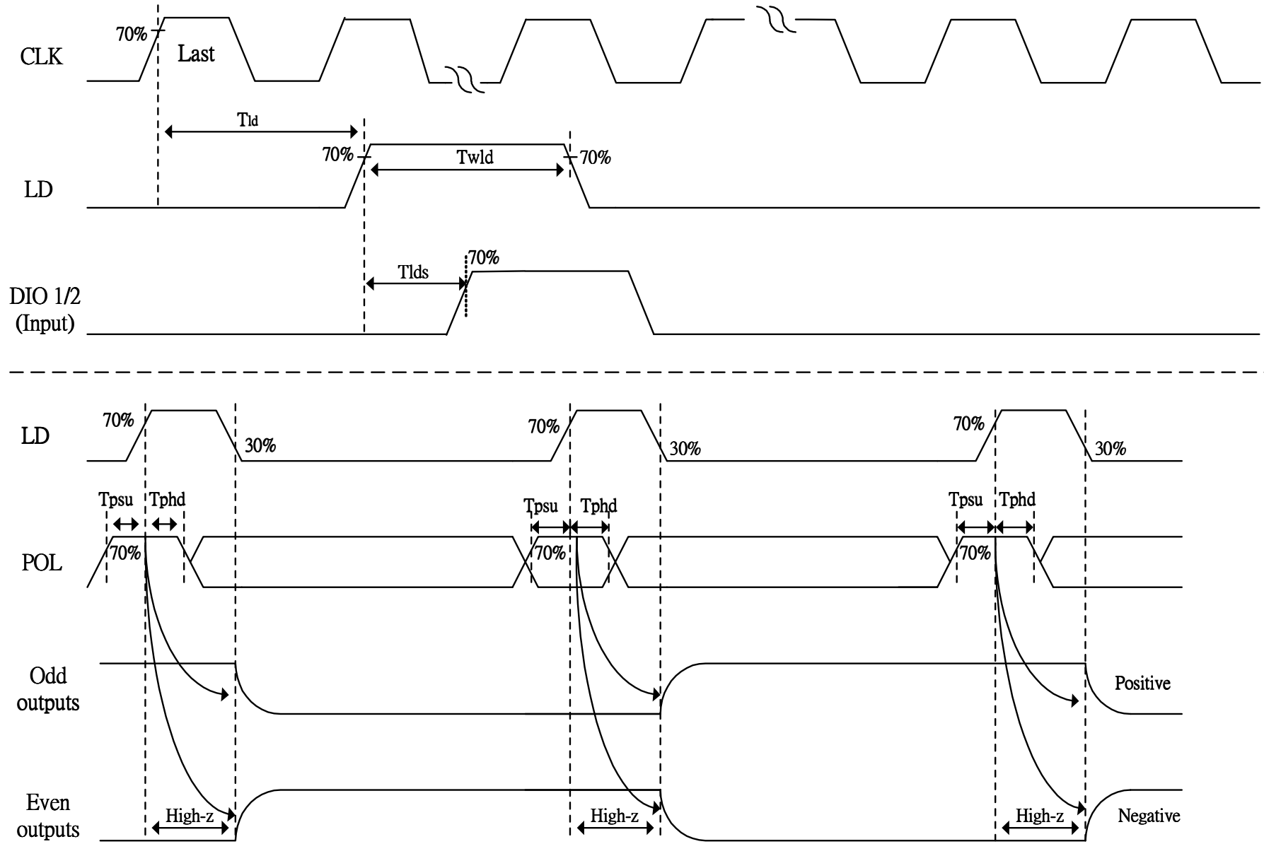
Fig. 11-2 Horizontal timing(2)
